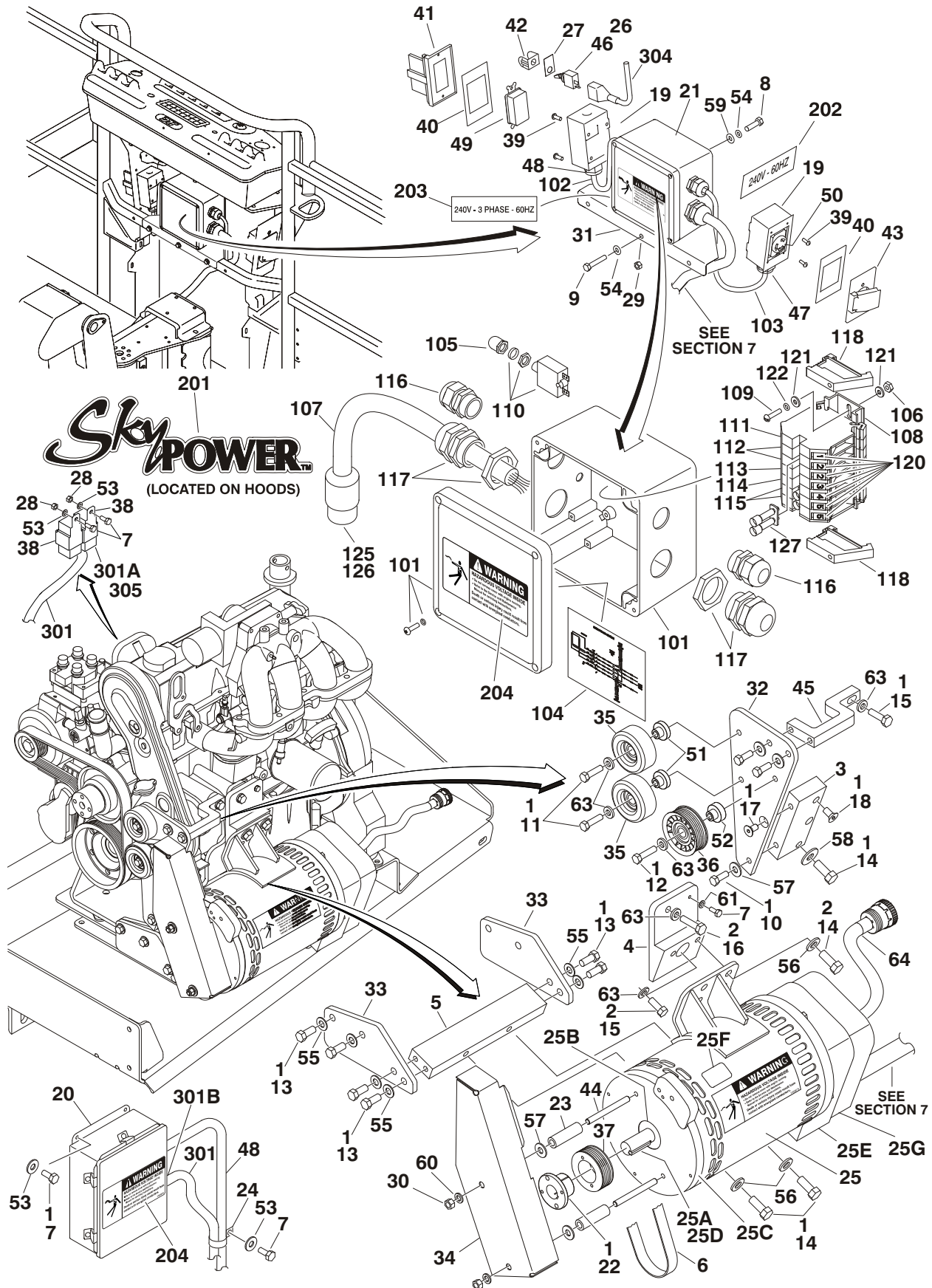
FIGURE 2-34. 7500W SKYPOWER GENERATOR INSTALLATION - FORD ENGINES
