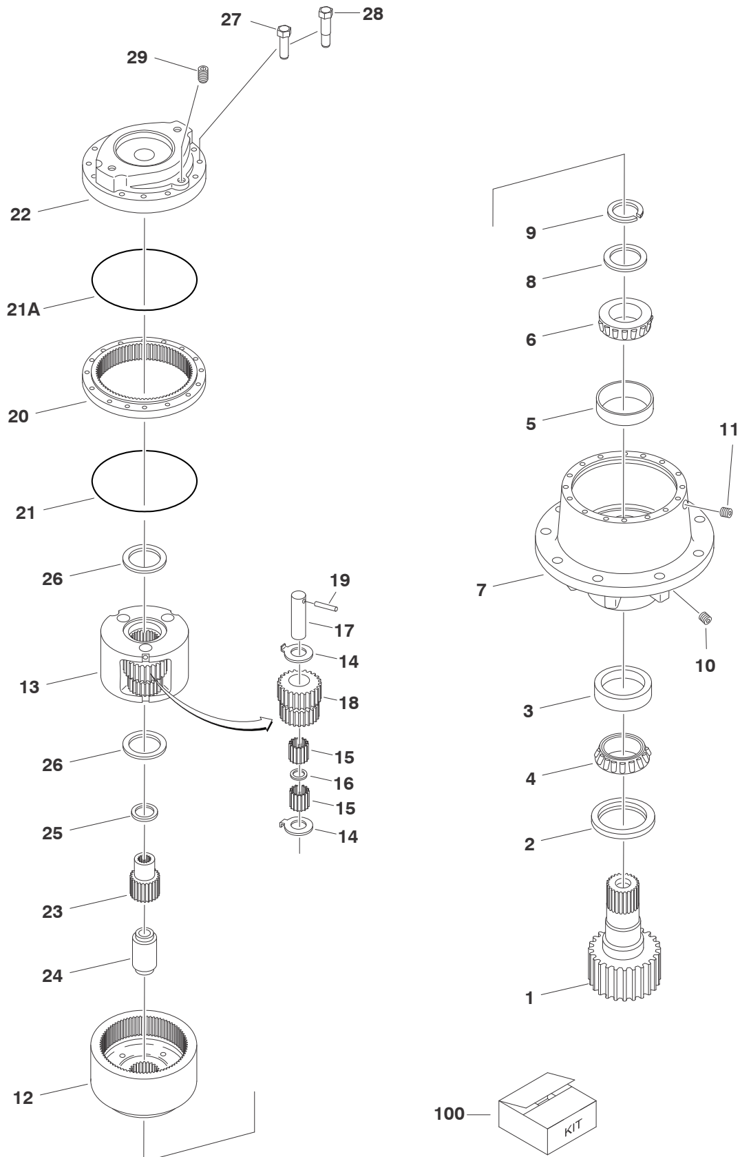
FIGURE 2-4. SWING HUB ASSEMBLY (PRIOR TO SN 0300066417)
