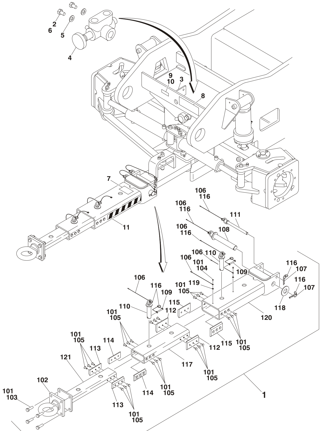
FIGURE 1-12. TOW PACKAGE INSTALLATION
