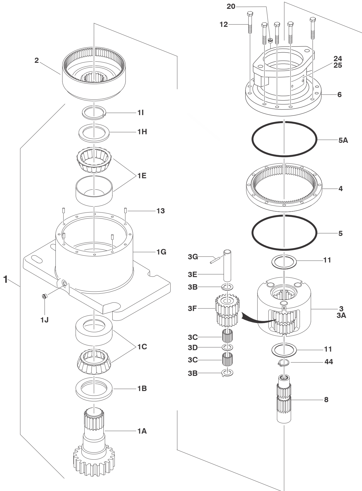
FIGURE 2-7. SWING MOTOR/HUB ASSEMBLY (SN 0300134352 TO SN 0300140000)
