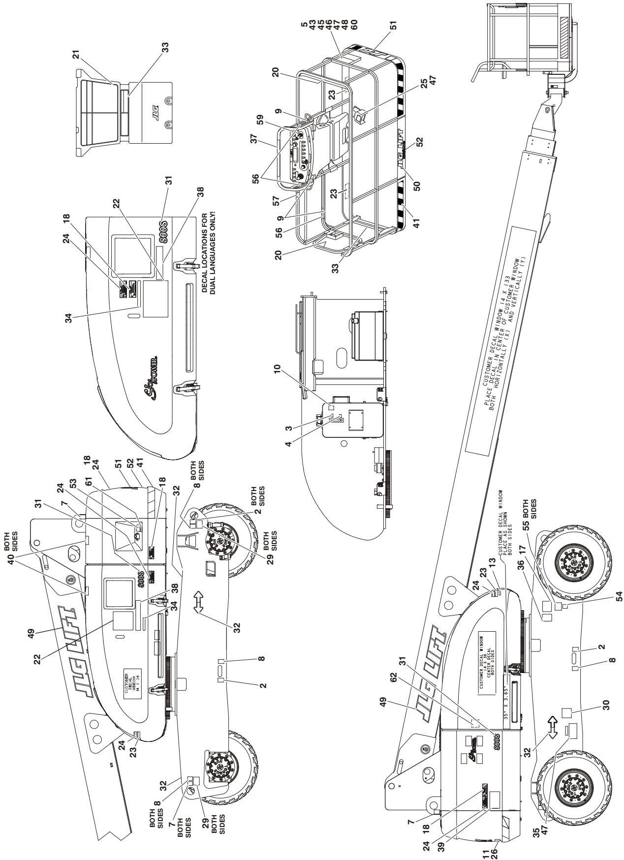
FIGURE 8-2. DECAL INSTALLATION (ANSI SPEC) (SN 0300088933 TO SN 0300140000)
