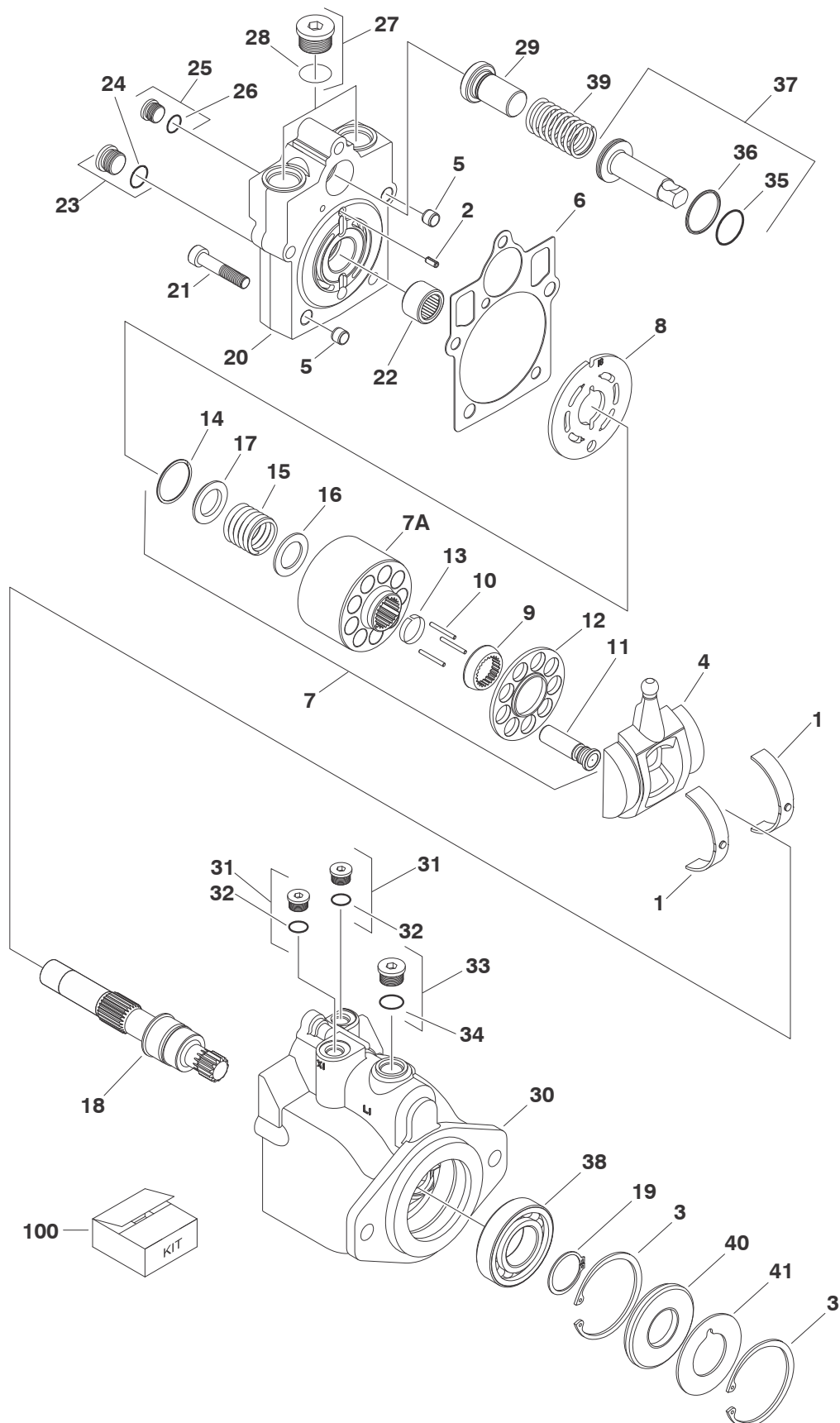
FIGURE 1-9. DRIVE MOTOR ASSEMBLY (5 BOLT ASSEMBLY)
