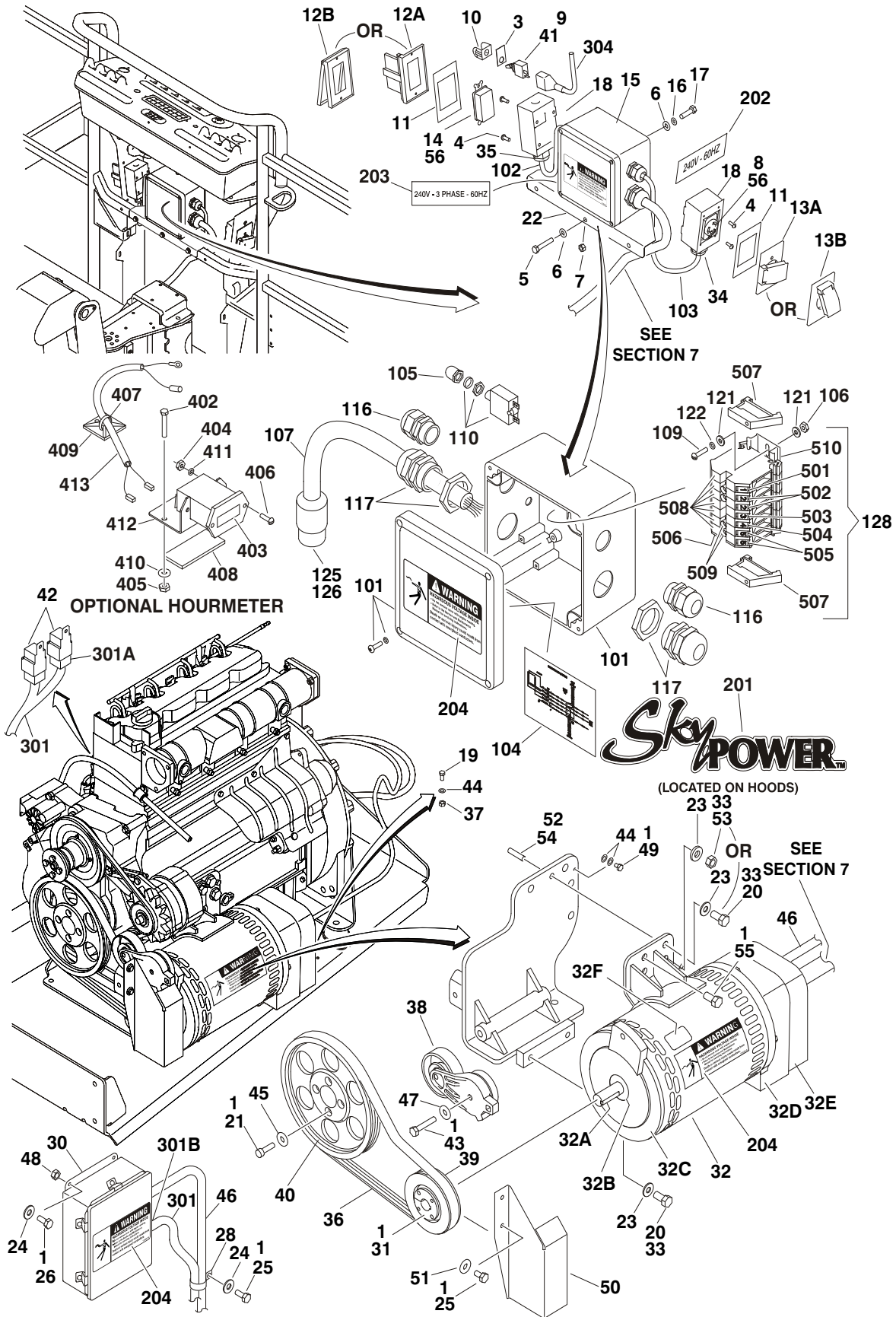
FIGURE 2-33. 7500W SKYPOWER GENERATOR INSTALLATION - CATERPILLAR & DEUTZ ENGINES
