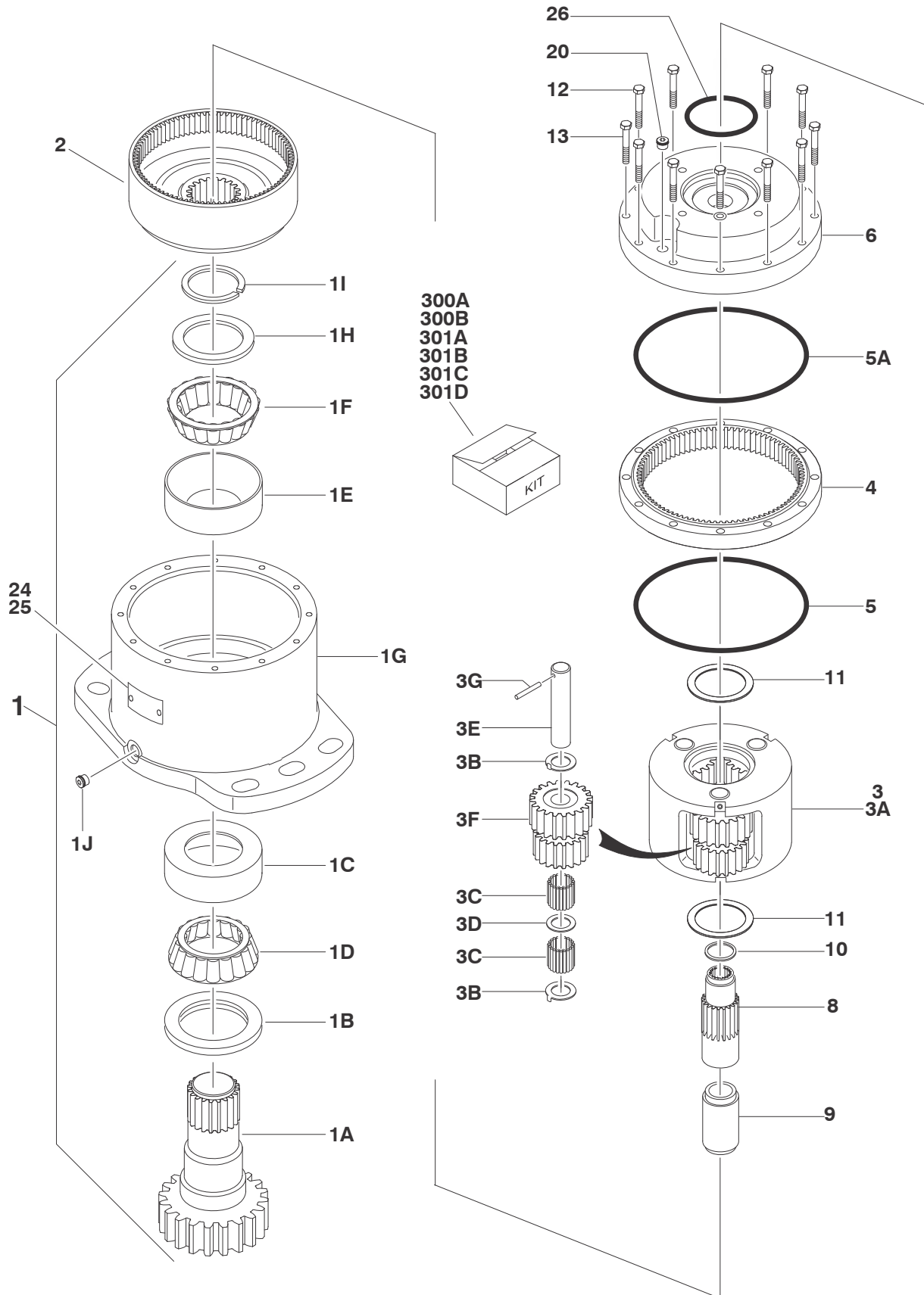
FIGURE 2-6. SWING MOTOR/HUB ASSEMBLY (SN 0300066417 TO SN 0300134352)
