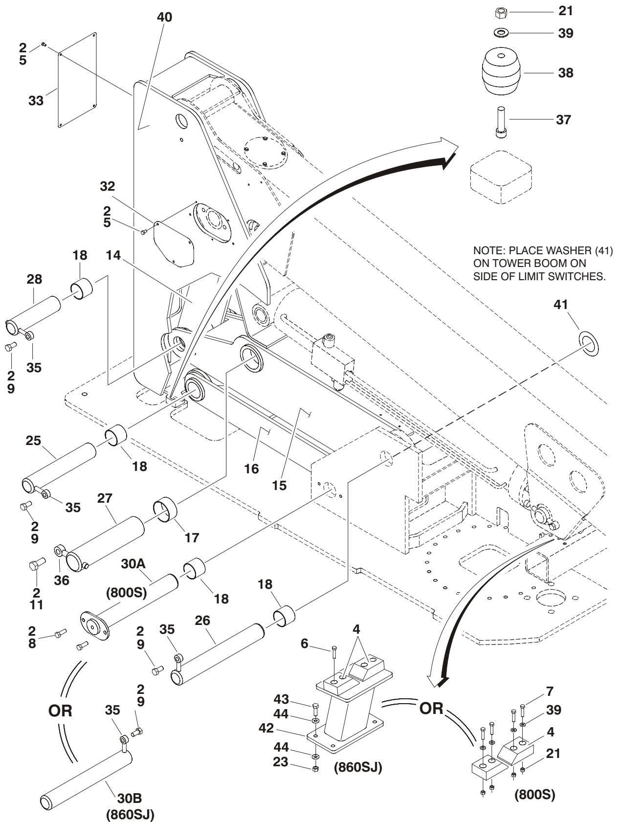
FIGURE 3-1. TOWER BOOM, UPRIGHT AND CYLINDERS INSTALLATION
