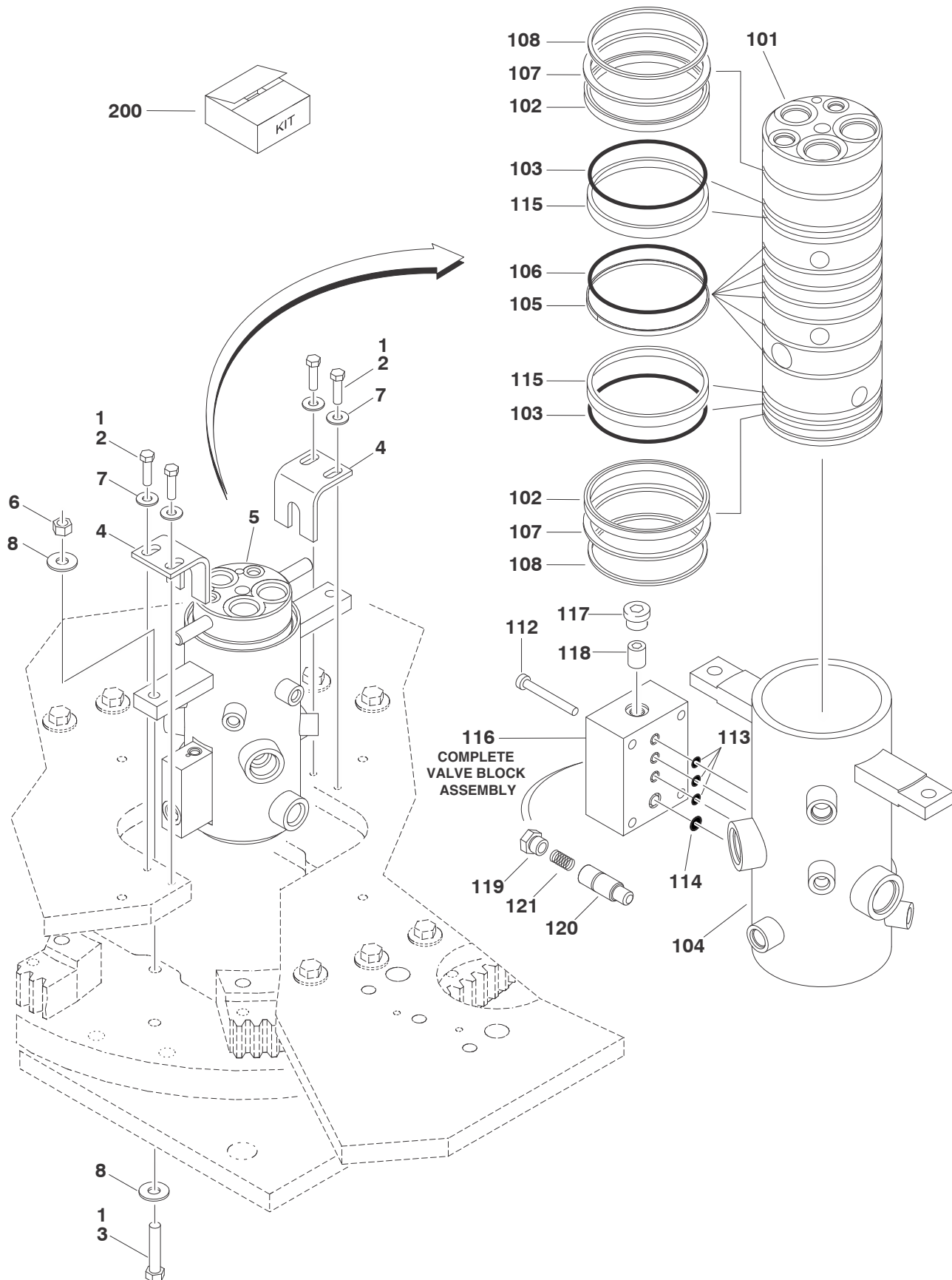
FIGURE 2-20. ROTARY COUPLING INSTALLATION (PRIOR TO SN 0300083331)
