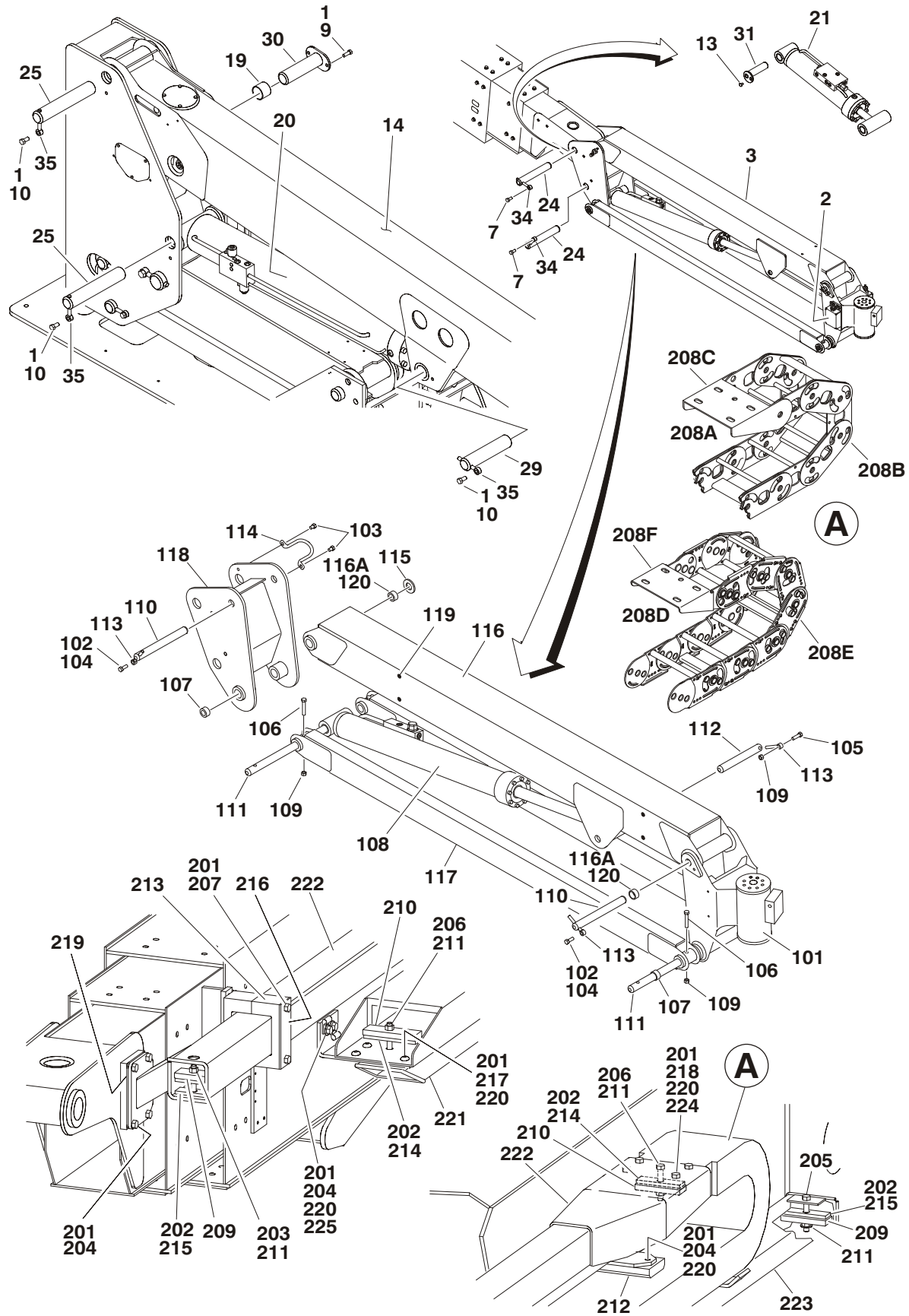
FIGURE 3-3. MAIN BOOM INSTALLATION - 860SJ
