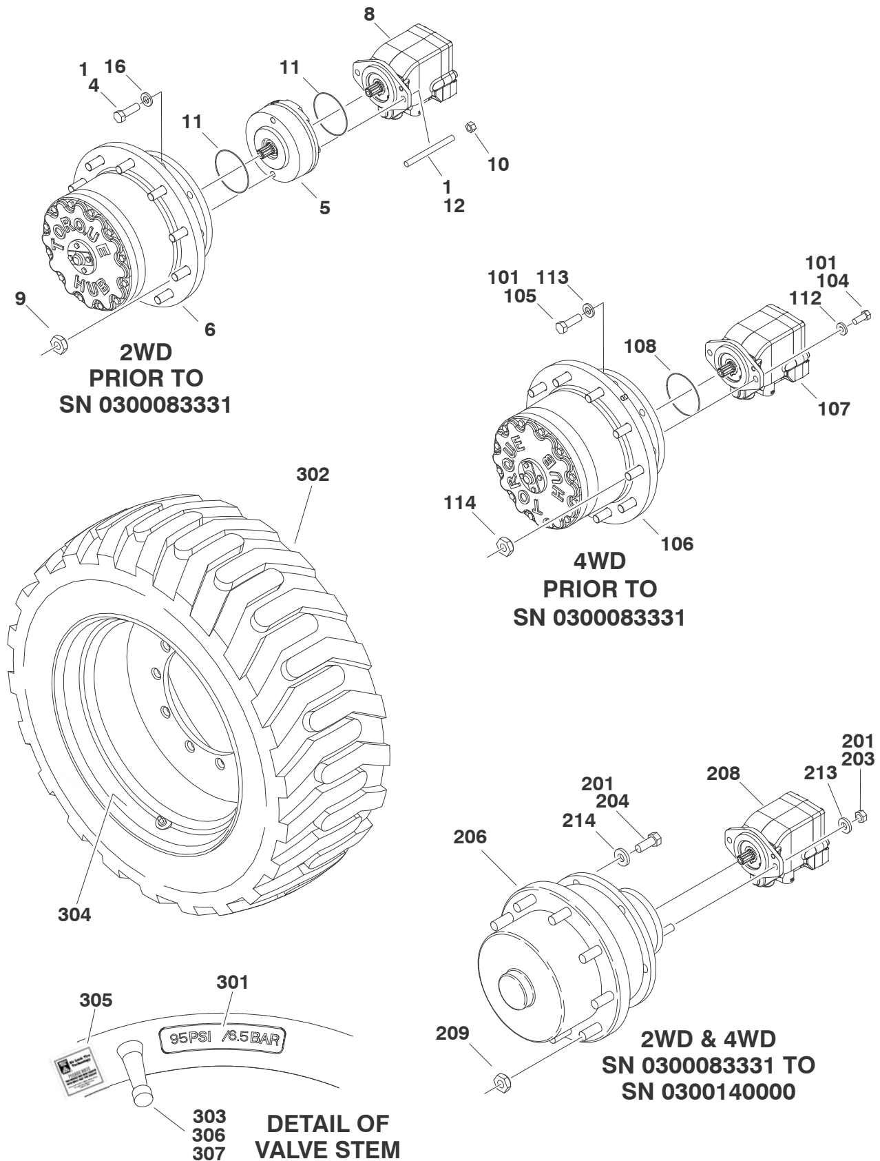
FIGURE 1-3. TIRE AND WHEEL DRIVE INSTALLATIONS
