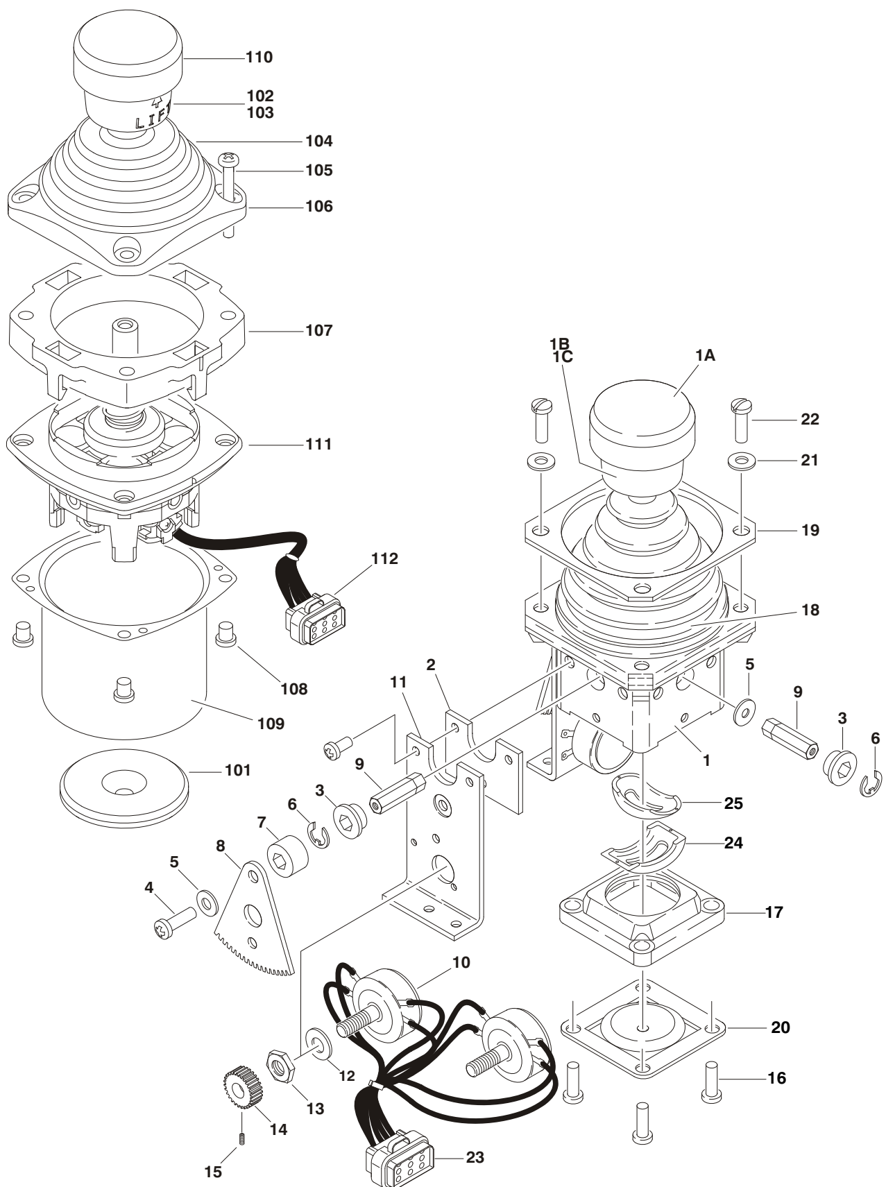
FIGURE 4-5. CONTROLLER ASSEMBLY (LIFT AND SWING)
