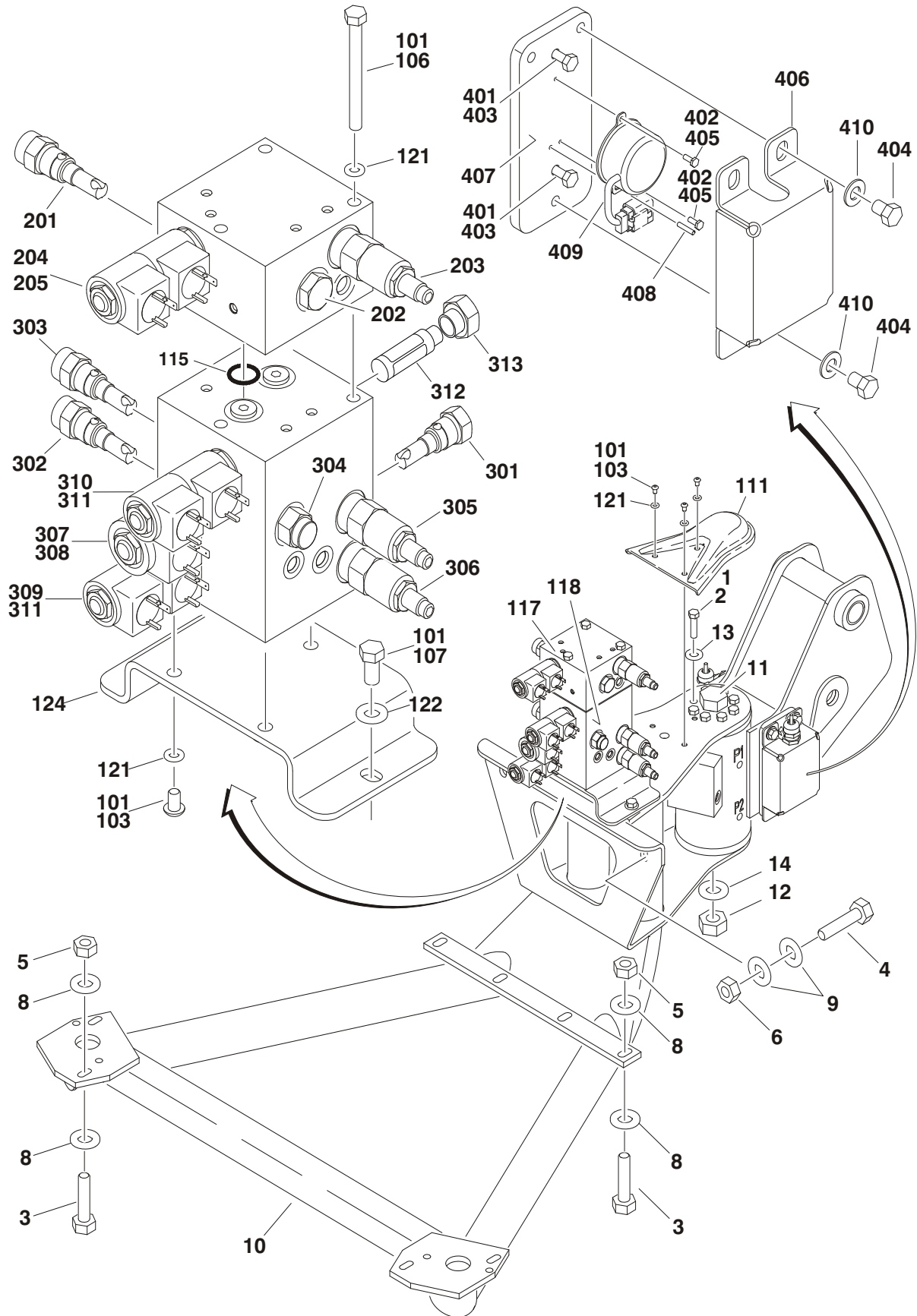
FIGURE 3-6. PLATFORM SUPPORT & CONTROL VALVES INSTALLATIONS
