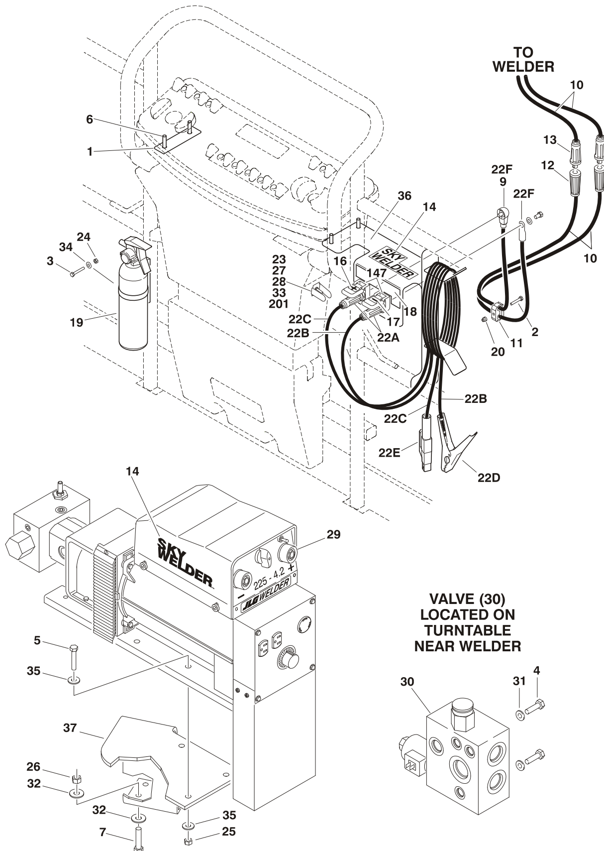
FIGURE 10-2. SKY WELDER INSTALLATION
