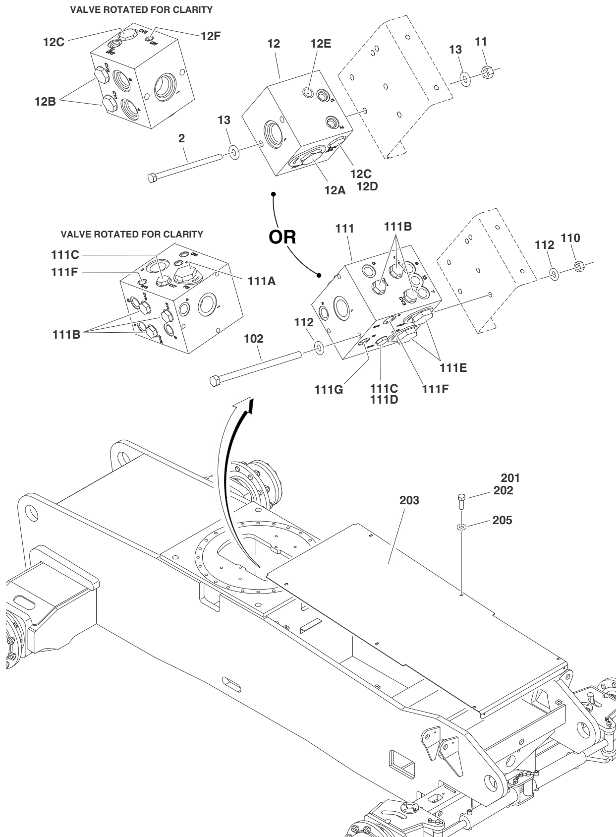
FIGURE 1-11. FRAME VALVES & SHIELDS INSTALLATIONS (SN 0300083331 TO SN 0300140000)
