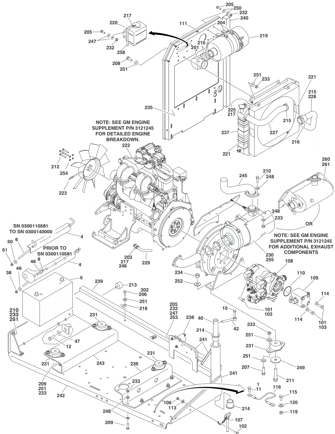
FIGURE 2-15. GM ENGINE INSTALLATION (PRIOR TO SN 0300139210)
