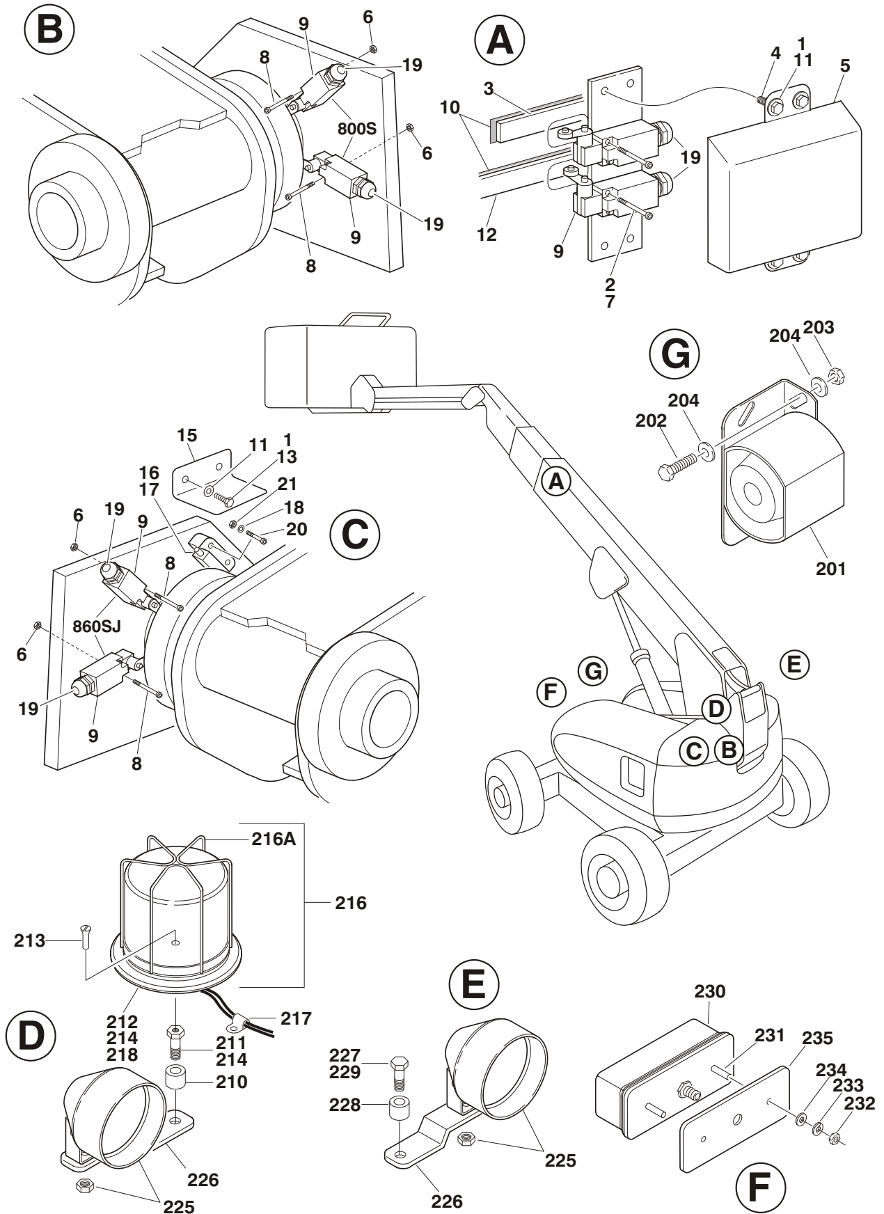
FIGURE 2-24. LIMIT SWITCHES, LIGHTS & ALARM INSTALLATIONS
