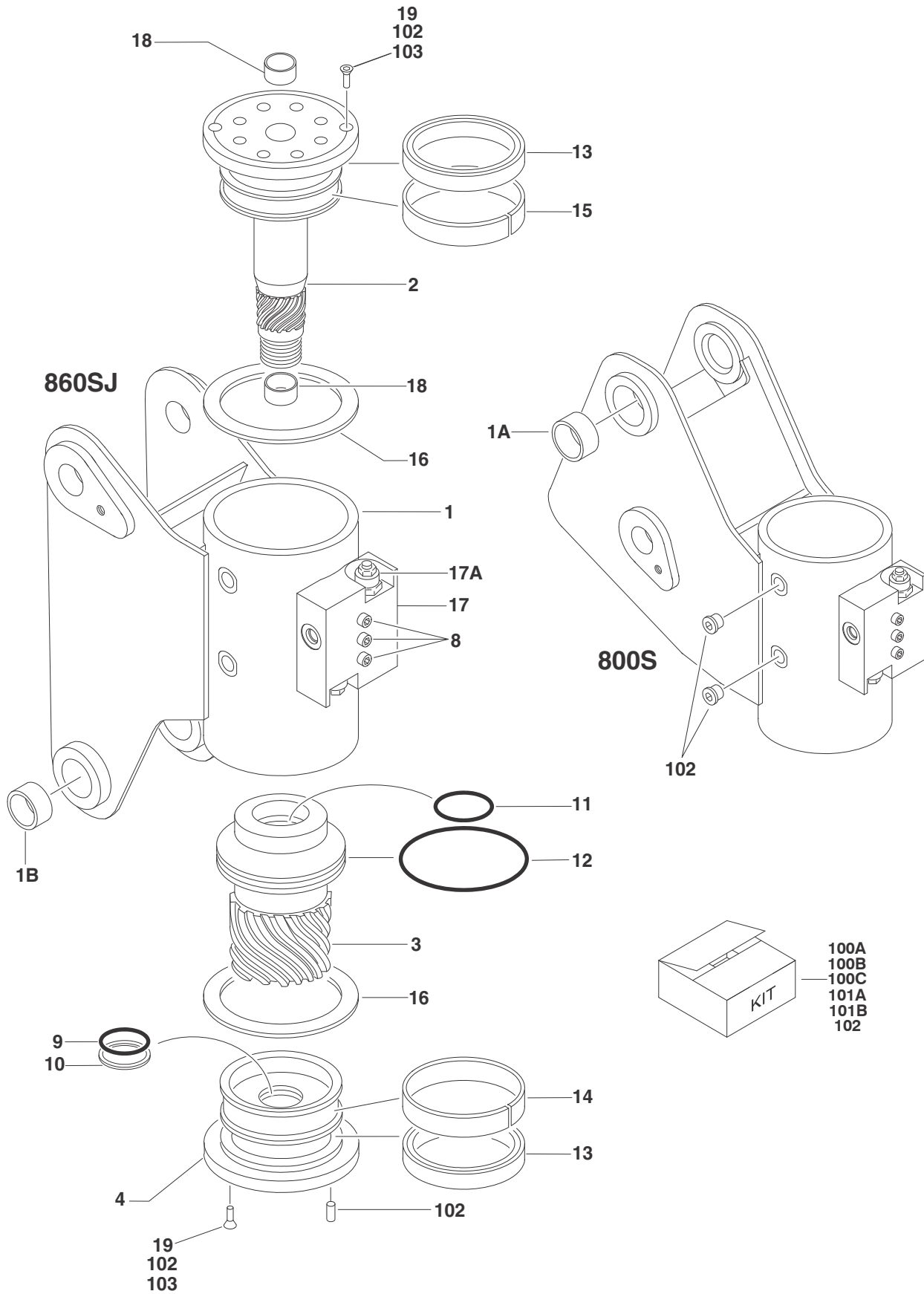
FIGURE 3-5. ROTATOR ASSEMBLY
