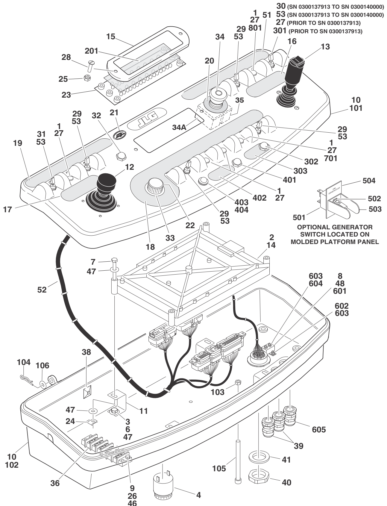
FIGURE 4-4. PLATFORM CONSOLE ASSEMBLY
