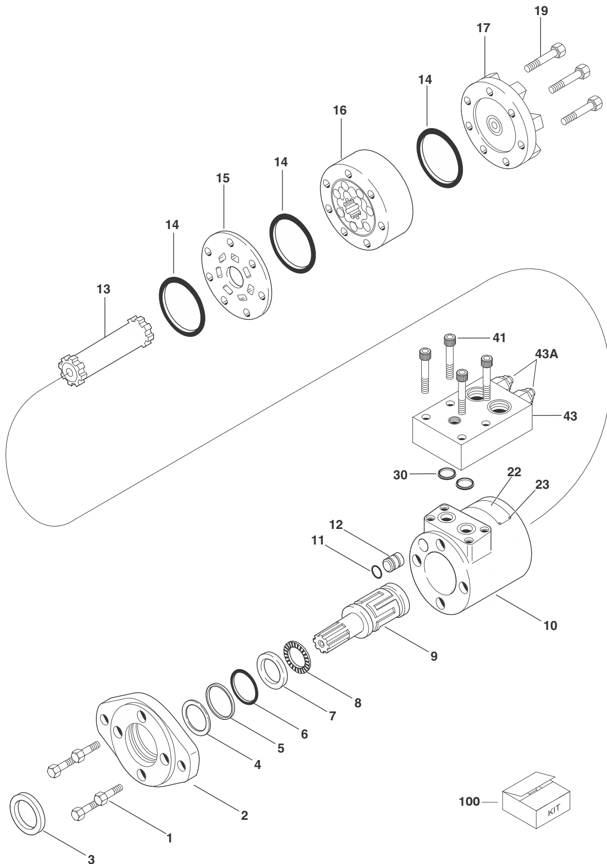
FIGURE 2-5. SWING MOTOR ASSEMBLY (PRIOR TO SN 0300066417)
