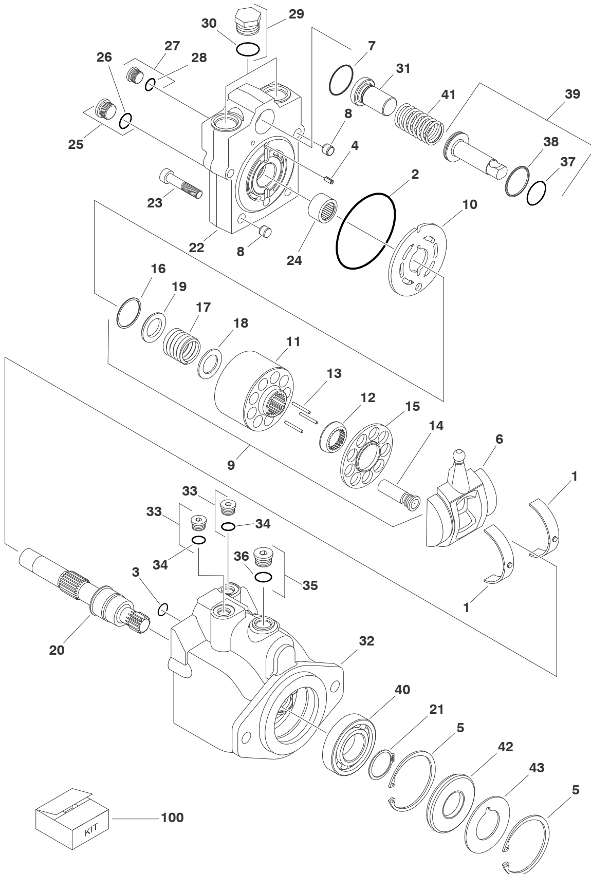
FIGURE 1-8. DRIVE MOTOR ASSEMBLY (2WD SN 0300083331 TO SN 0300098641 & ALL 4WD MACHINES) (4 BOLT ASSEMBLY)
