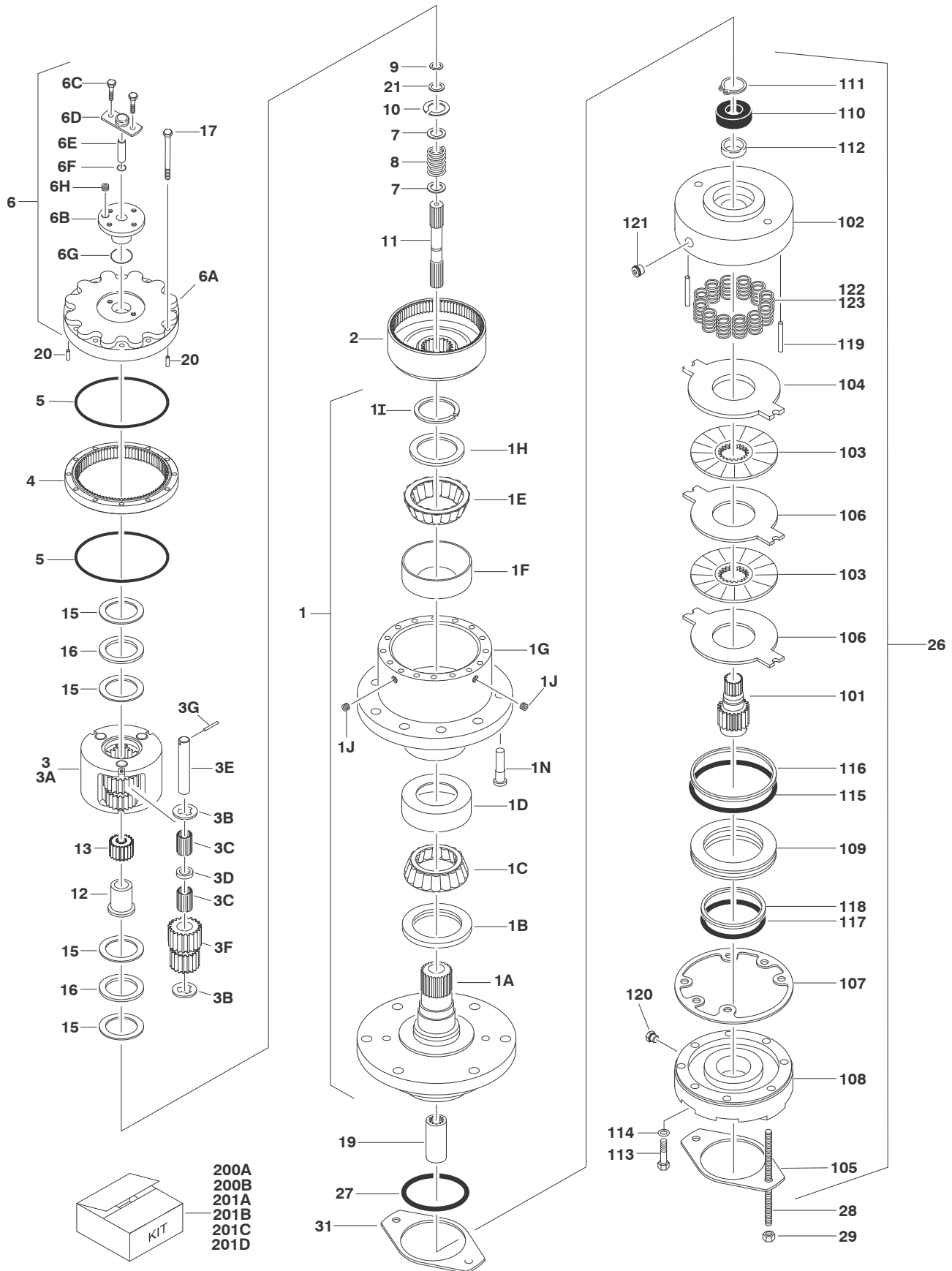
FIGURE 1-6. DRIVE HUB/BRAKE ASSEMBLY (SN 0300083331 TO SN 0300140000)
