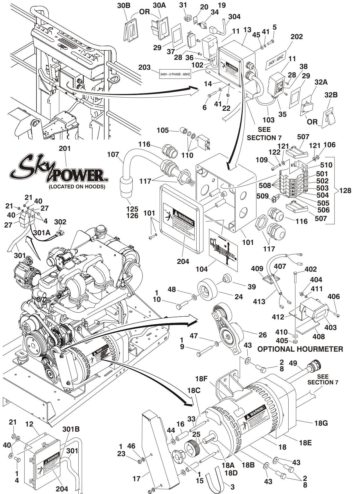
FIGURE 2-35. 7500W SKYPOWER GENERATOR INSTALLATION - GM ENGINES
