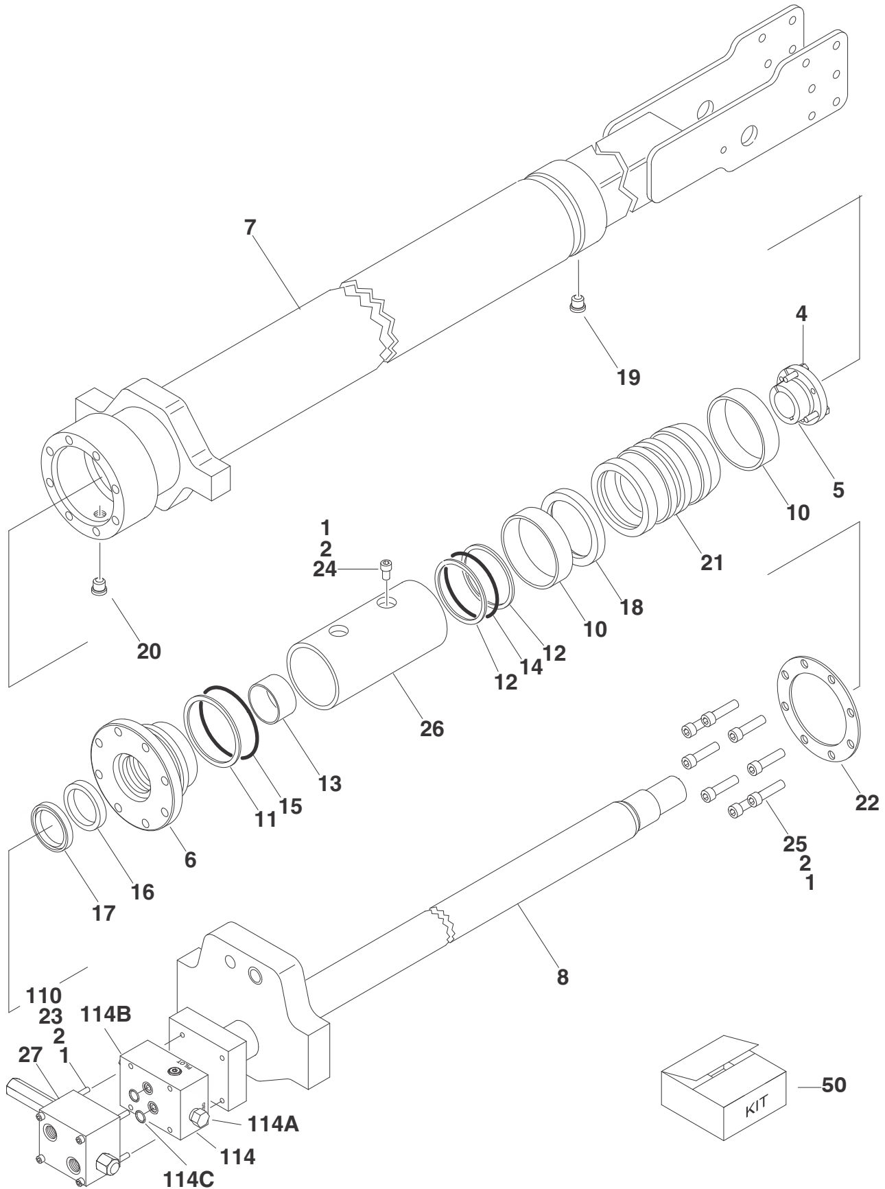
FIGURE 5-6. TELESCOPE CYLINDER ASSEMBLY
