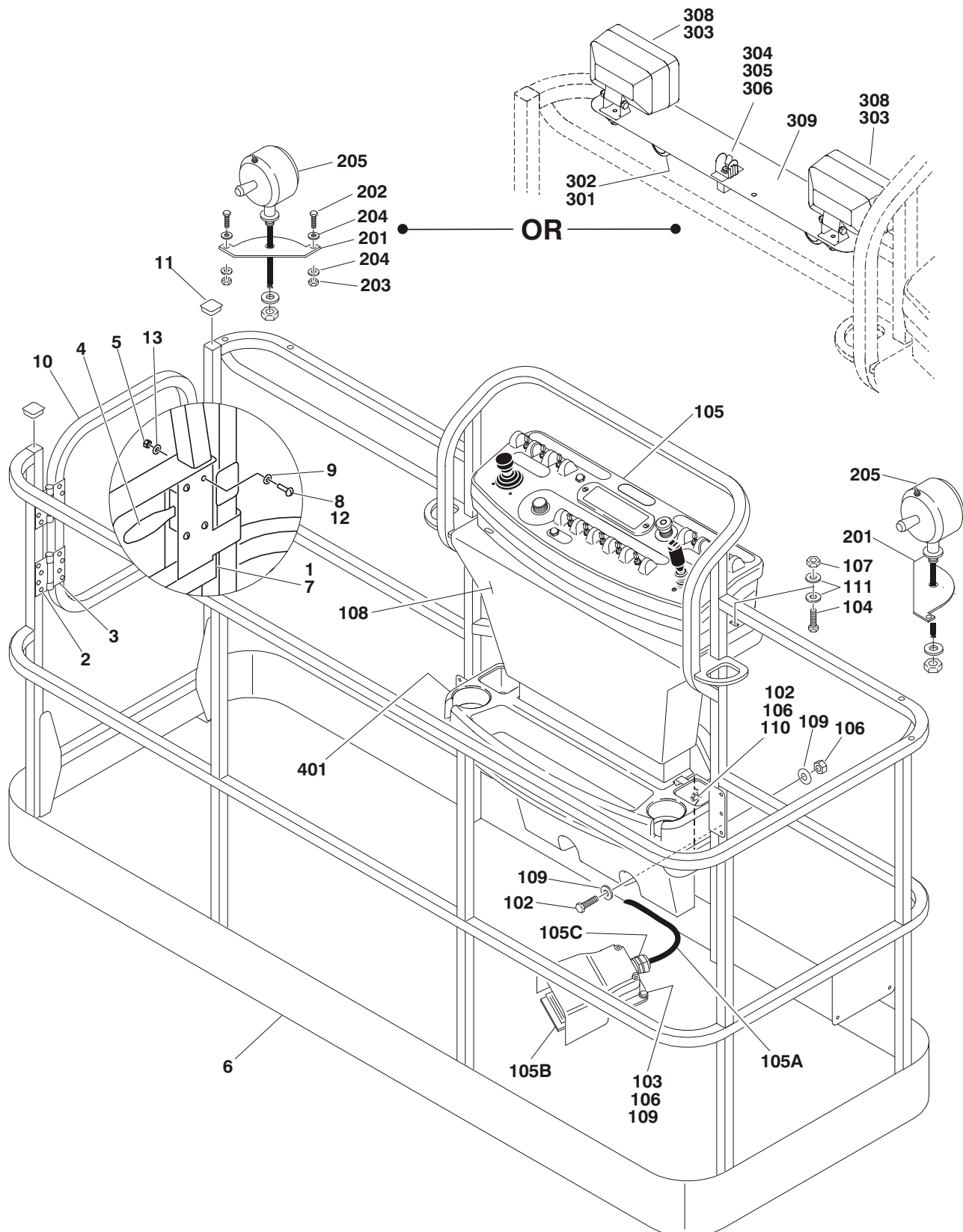
FIGURE 4-2. PLATFORM ASSEMBLIES - SIDE ENTRY (SN 0300067916 TO SN 0300140000)
