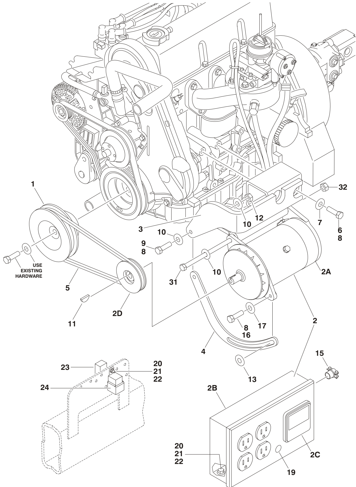
FIGURE 2-30. 2500W GENERATOR INSTALLATION - FORD MACHINES (PRIOR TO SN 03000079612) (OPTIONAL)
