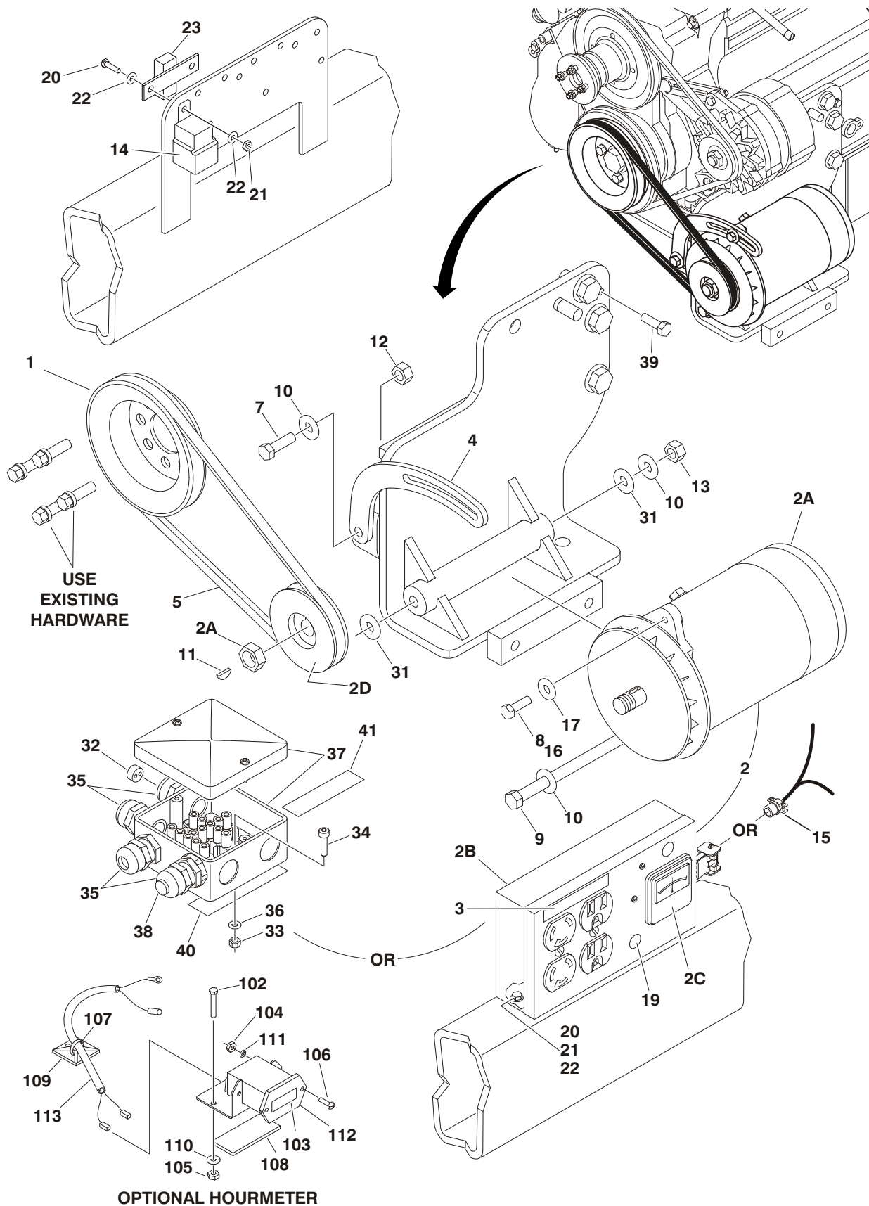
FIGURE 2-29. 2500W GENERATOR INSTALLATION - DEUTZ MACHINES (OPTIONAL)
