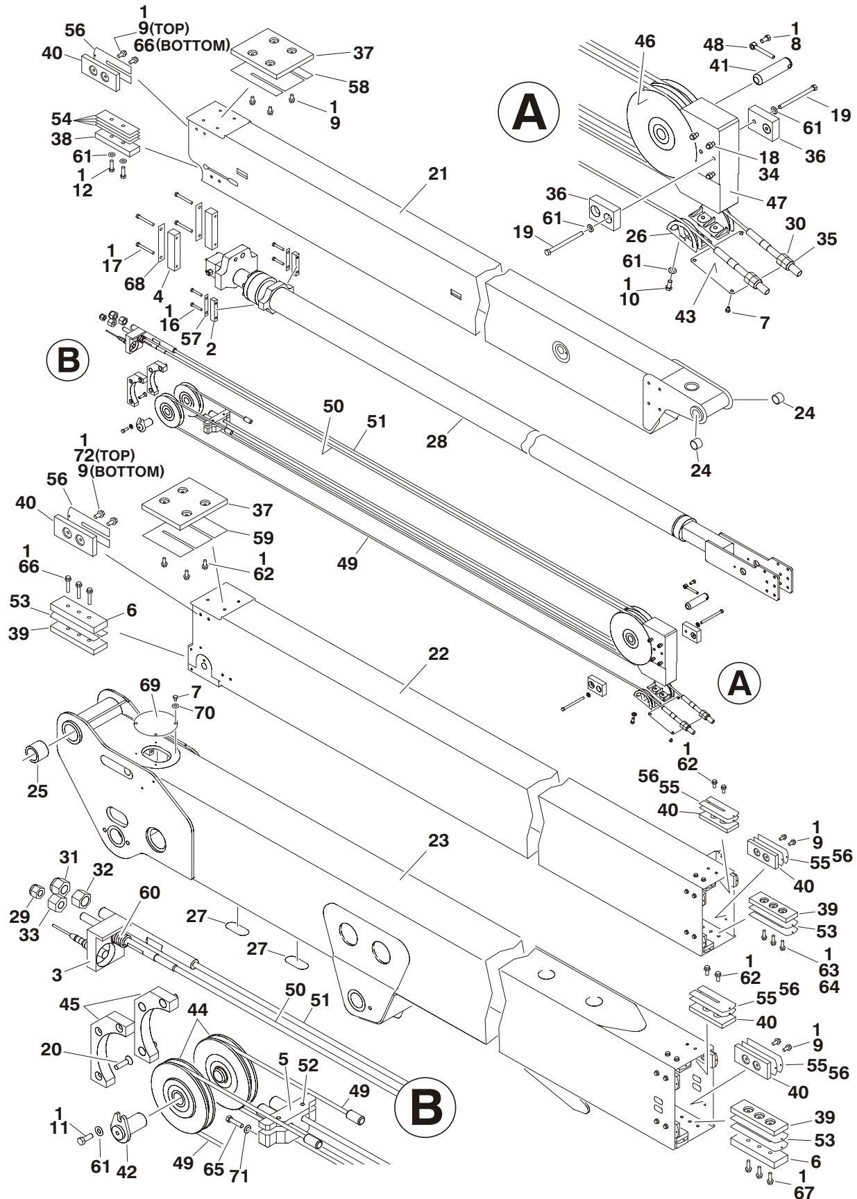
FIGURE 3-4. MAIN BOOM ASSEMBLY
