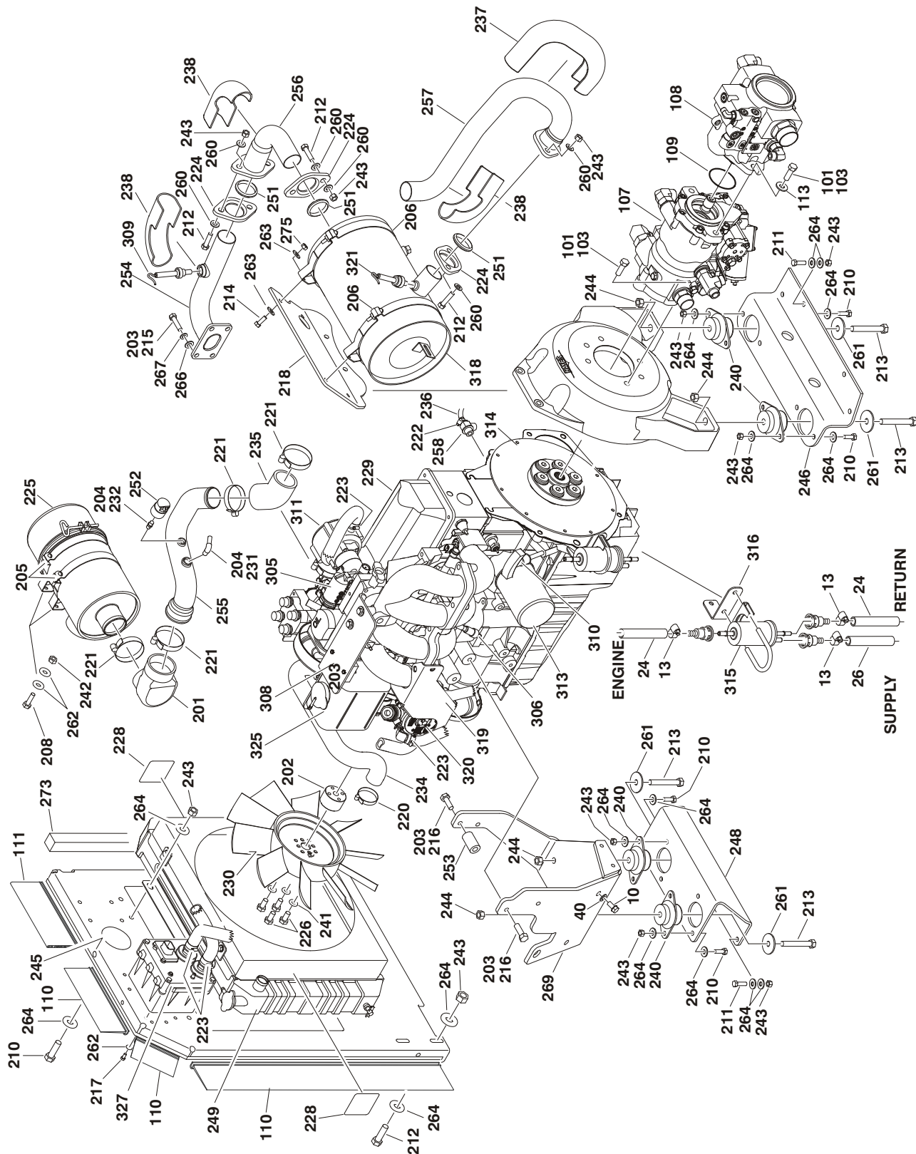
FIGURE 2-13. FORD ENGINE INSTALLATION (SN 0300079612 TO SN 0300140000)
