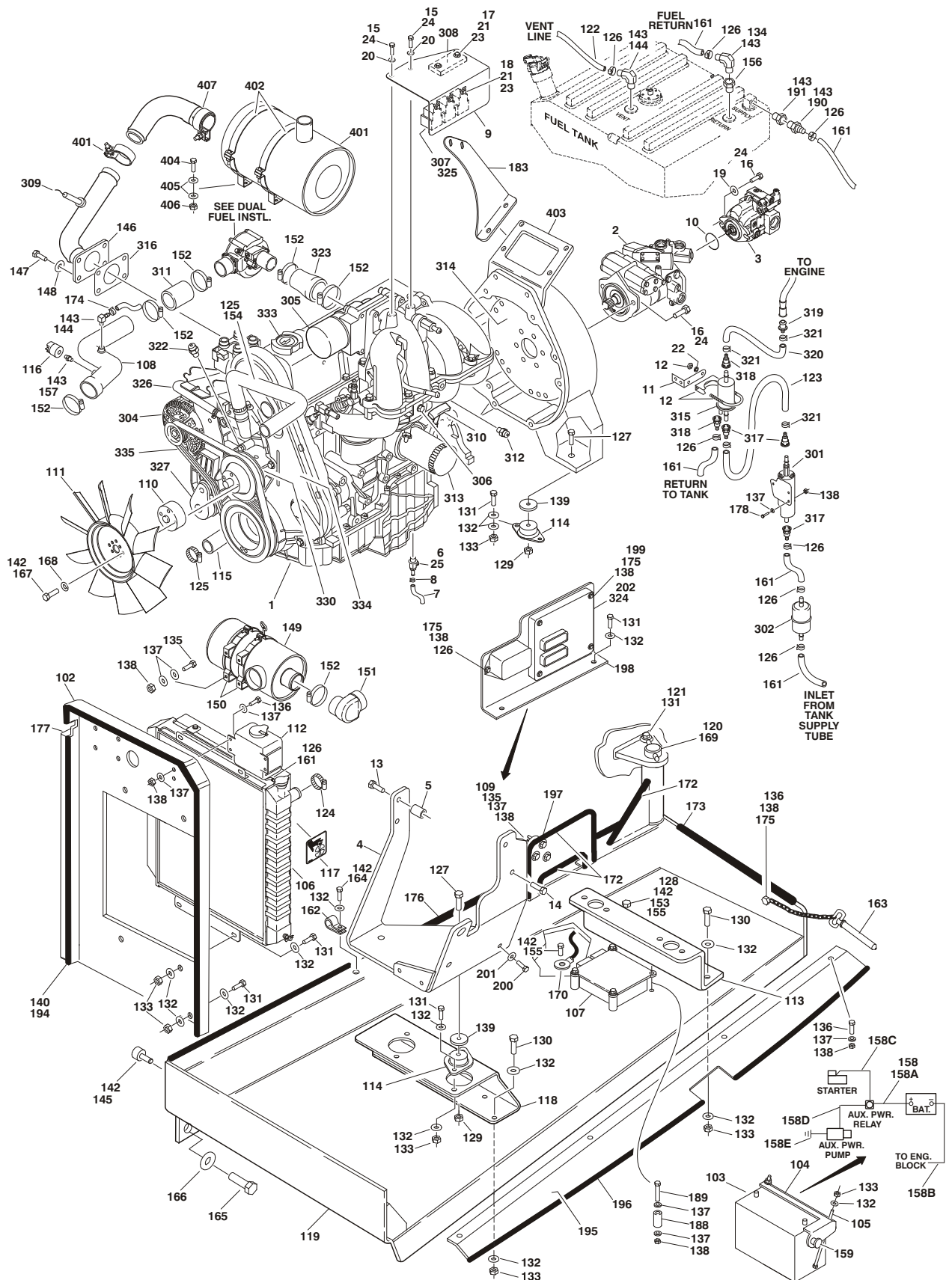
FIGURE 2-12. FORD ENGINE INSTALLATION (PRIOR TO SN 0300079612)
