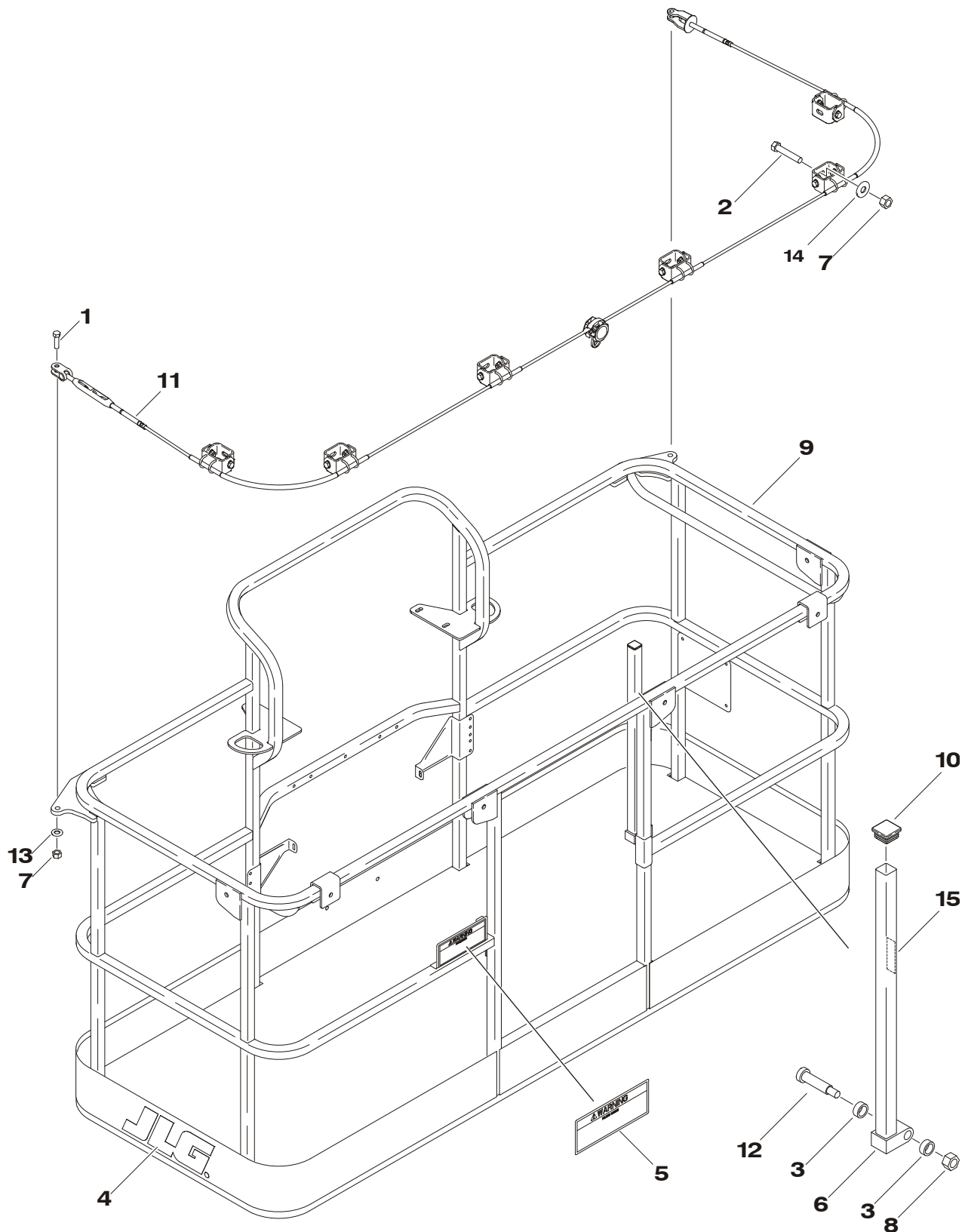
FIGURE 4-3. PLATFORM COMPONENTS INSTALLATION (FALL ARREST PLATFORM)
