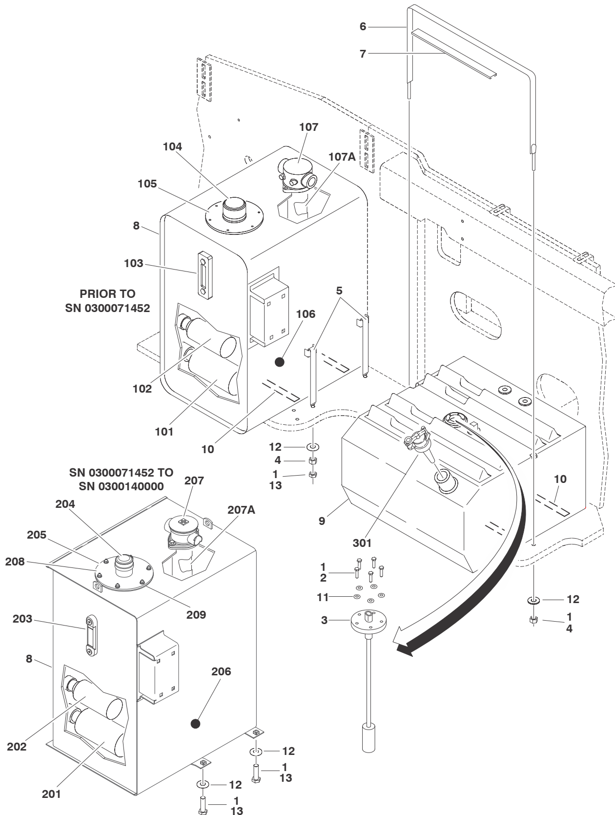
FIGURE 2-19. TANK INSTALLATIONS
