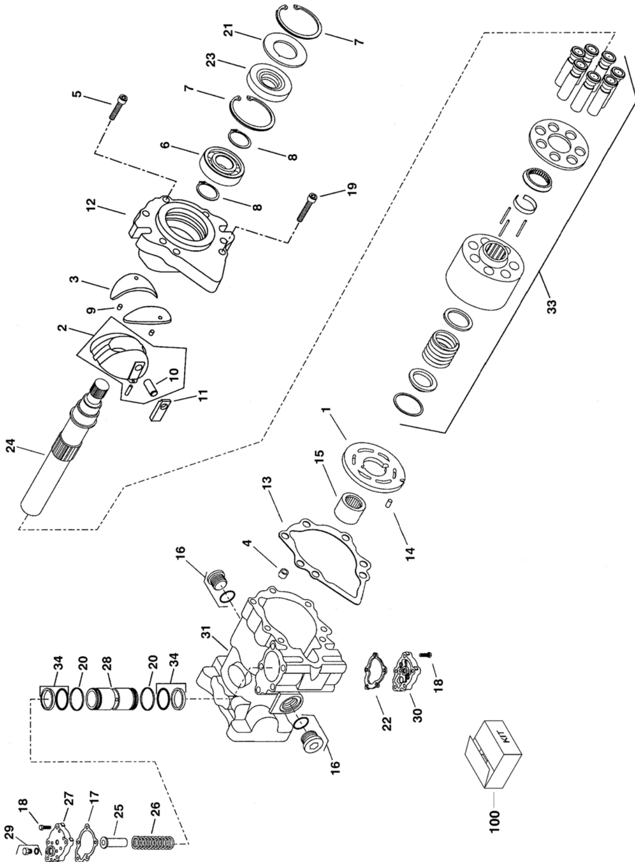
FIGURE 1-7. DRIVE MOTOR ASSEMBLY (2WD PRIOR TO SN 0300083331)
