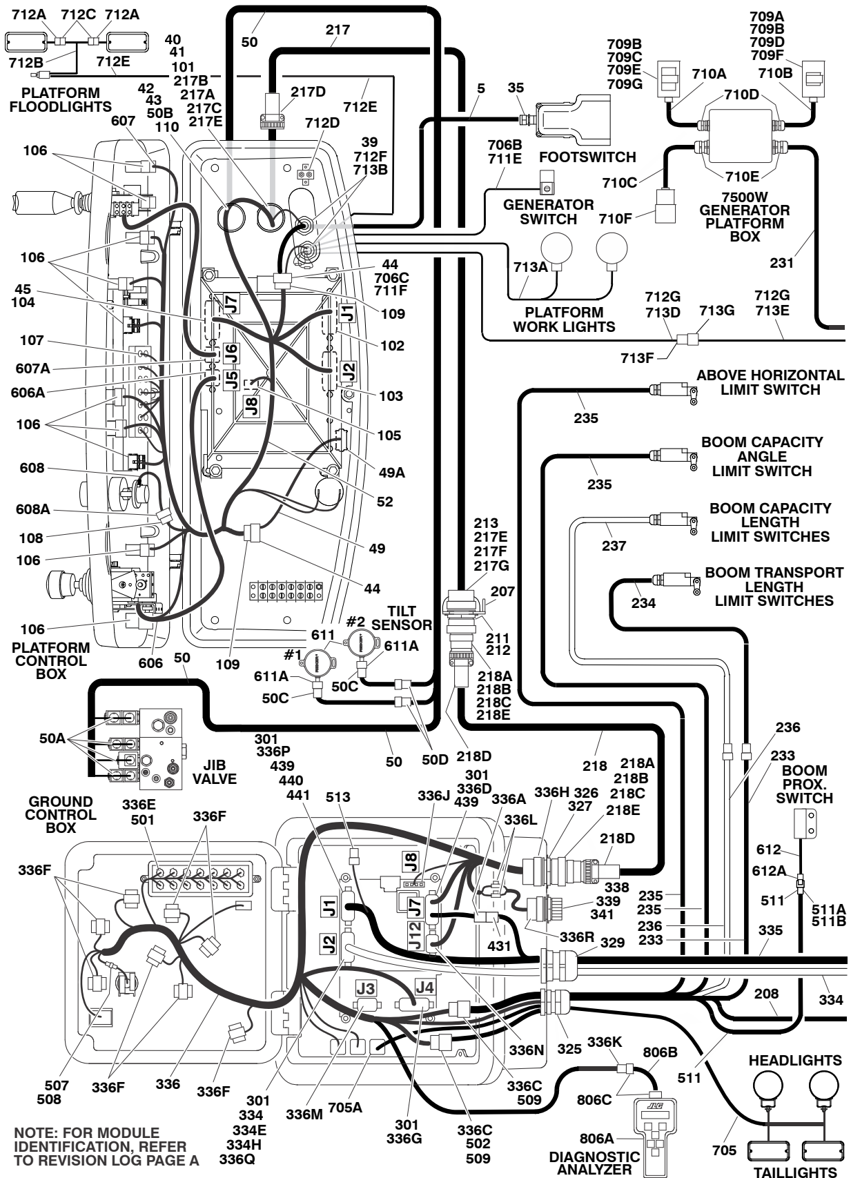
FIGURE 7-4. HARNESS COMPONENTS INSTALLATION (WITH UGM)
