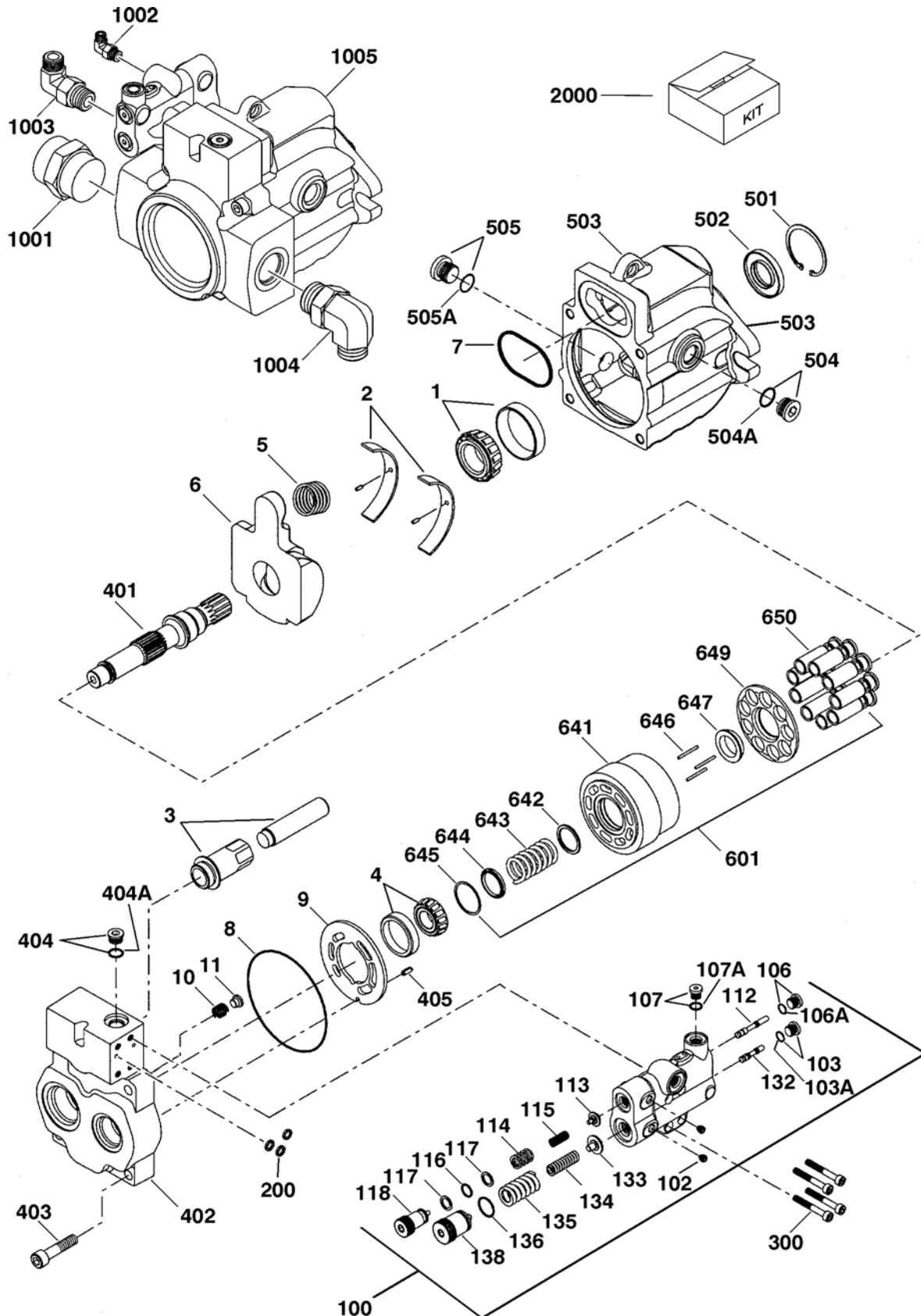
FIGURE 2-18. LOAD SENSING PUMP ASSEMBLY
