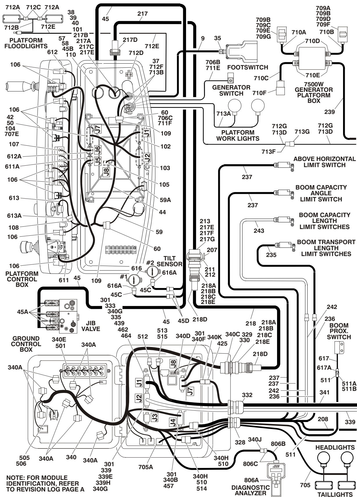
FIGURE 7-3. HARNESS COMPONENTS INSTALLATION (WITHOUT UGM) (SN 0300085332 TO SN 0300140000)
