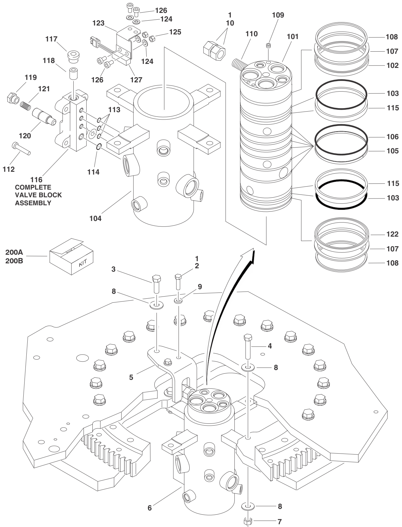
FIGURE 2-21. ROTARY COUPLING INSTALLATION (SN 0300083331 TO SN 0300140000)
