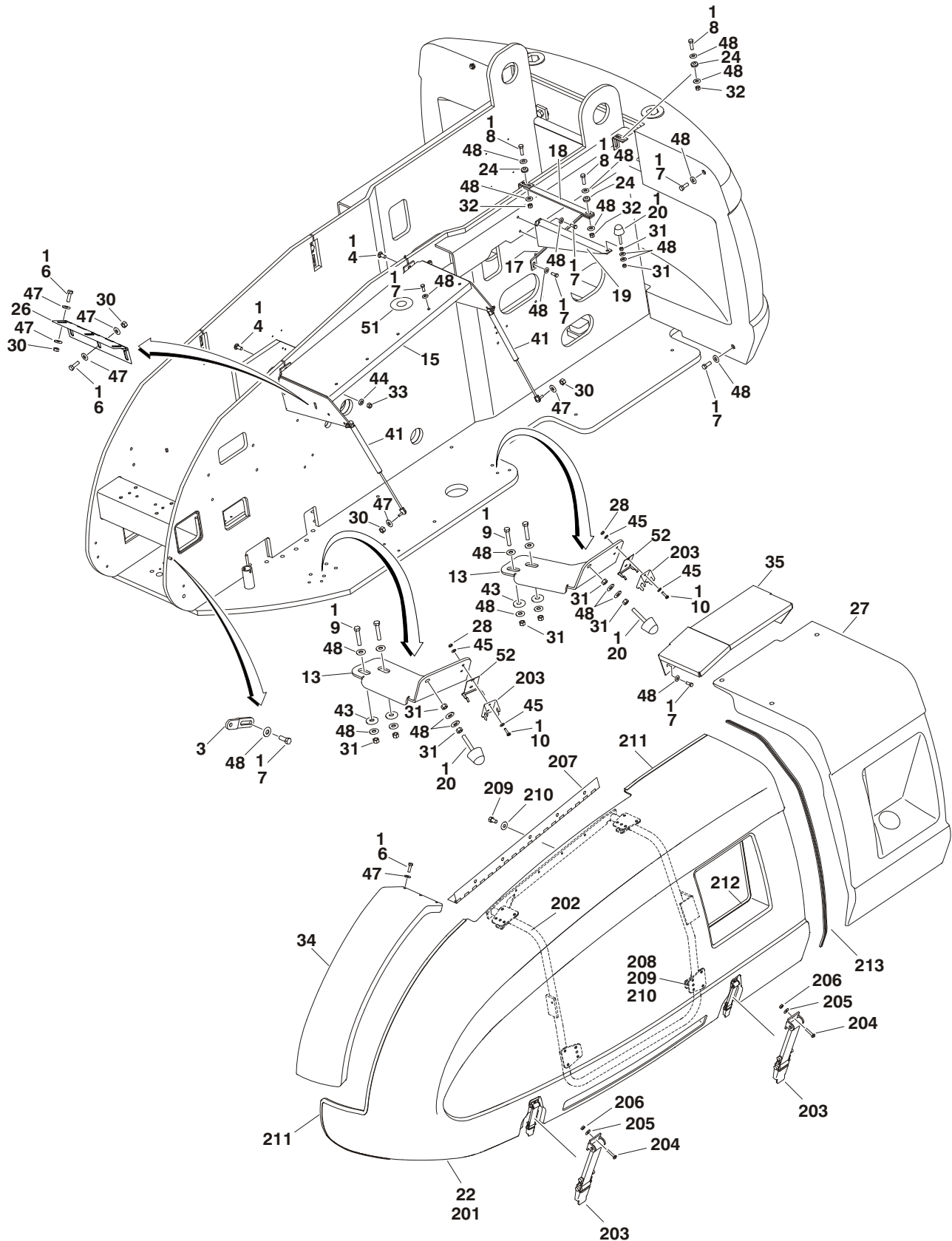
FIGURE 2-26. HOODS INSTALLATION (SN 0300089982 TO SN 0300140000)
