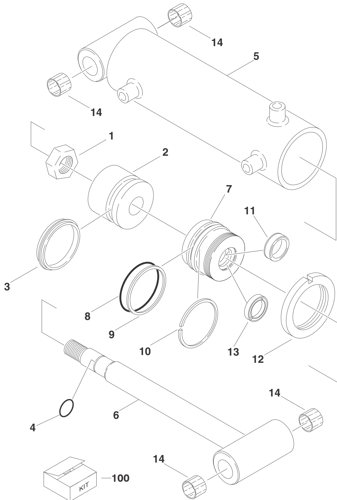
FIGURE 5-5. STEER CYLINDER ASSEMBLY
