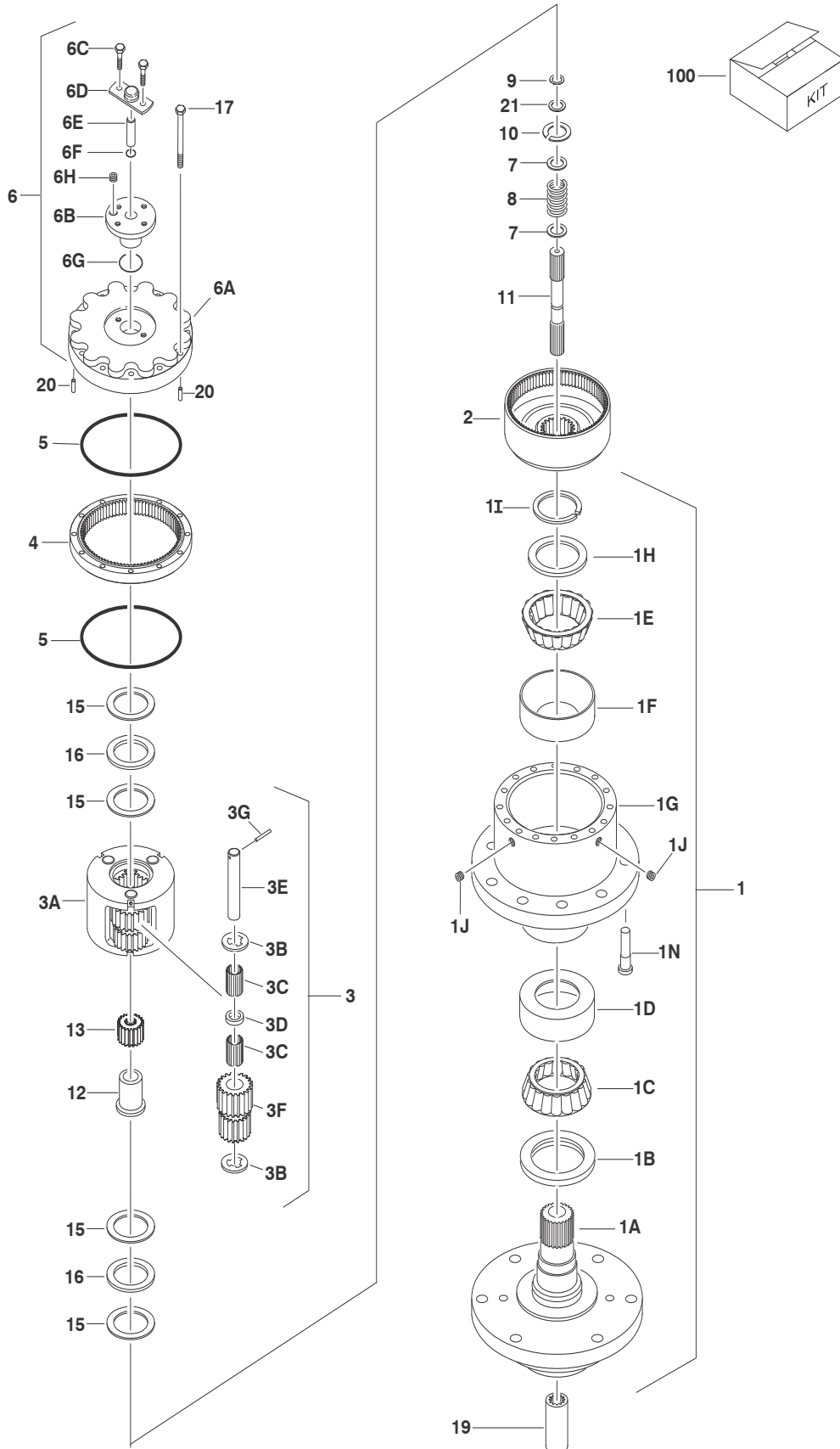
FIGURE 1-4. DRIVE HUB ASSEMBLY (2WD PRIOR TO SN 0300083331)
