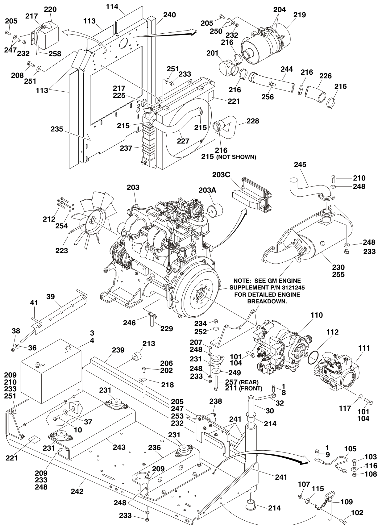
FIGURE 2-16. GM ENGINE INSTALLATION (SN 0300139210 TO SN 0300140000)
